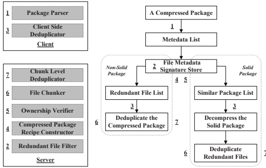
Fig. 2: Z-Dedup’s main modules and workflow.
