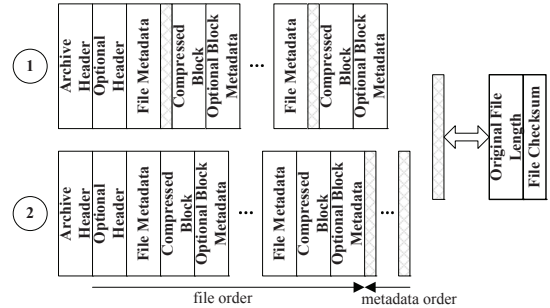
Fig. 4: Extending data layout of a compressed package.
